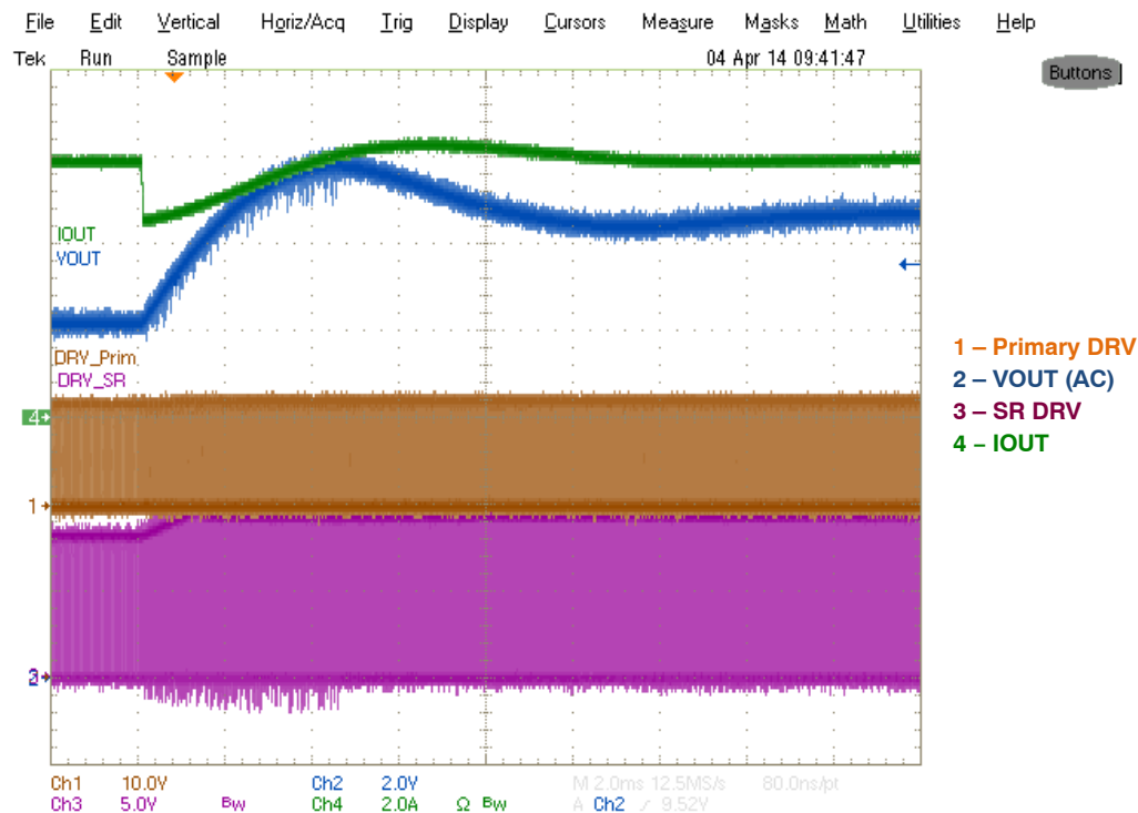
Figure 29. V_{IN} = 230 V_{AC} , I_{OUT} = 8.0\text{--}10.5 A
