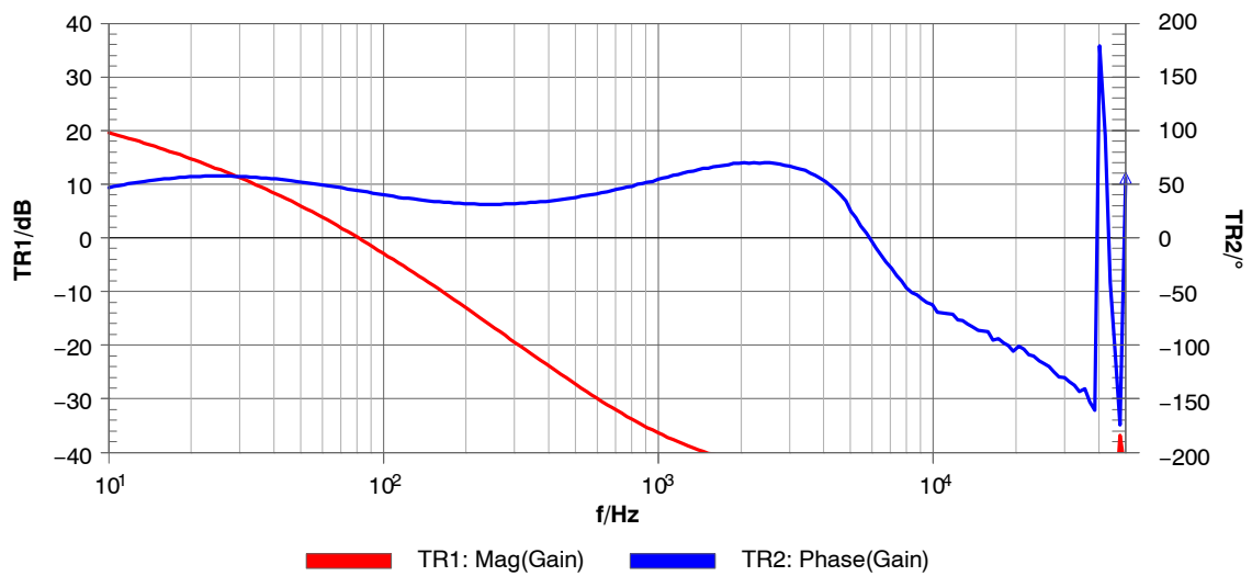
Figure 42. V_{\text{IN}} = 230 \text{ V}_{\text{AC}} , I_{\text{OUT}} = 5.9 \text{ A} , V_{\text{OUT}} = 8 \text{ V}
