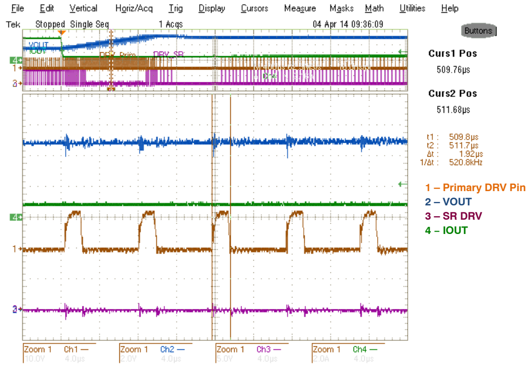
Figure 32. V_{IN} = 230 \text{ V}_{AC} , R_{OUT} = 1.5 \Omega to 10 \Omega – Detail Shows why SR is Not Turned On. It is Not Turned-on, because Primary On-time is Shorter than Secondary Side Min-off Time (in CCM they Correspond Each Other)
