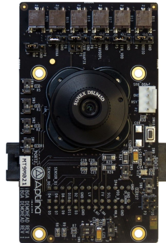
Figure 1. MT9M021 Evaluation Board
