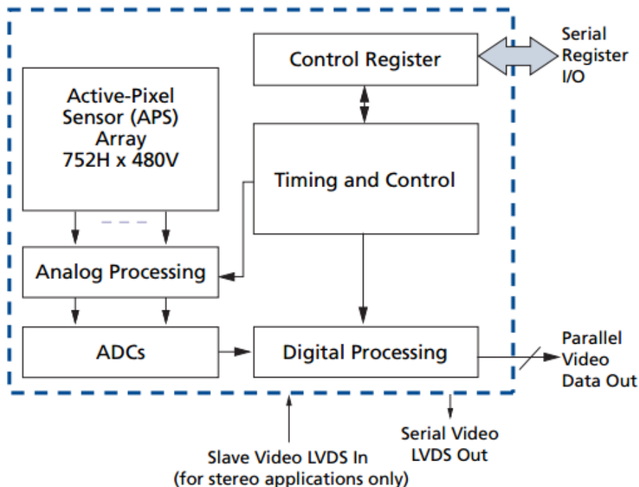
Figure 2. Block Diagram of MT9V034C12STMH-GEVB
