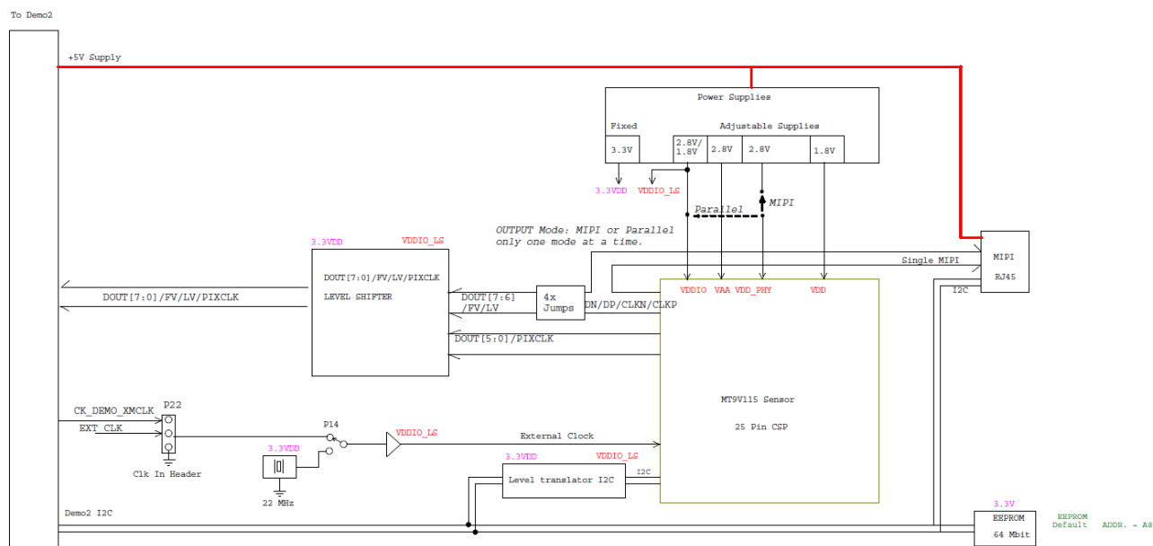
Figure 2. Block Diagram of MT9V115EBKSTCD-GEVB
