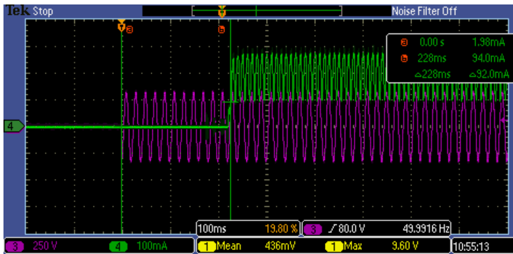
Figure 13. Start Up with AC Applied 230 V
