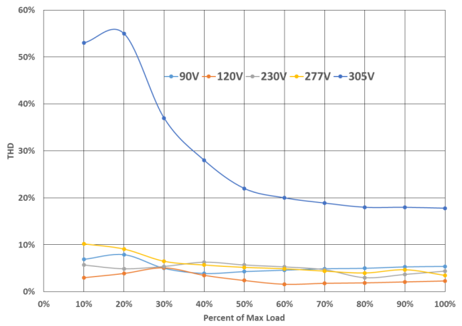
Figure 12. THDi
