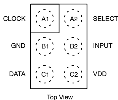
Figure 5. Pin Configuration
