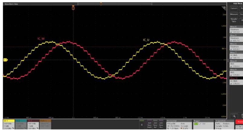
Figure 15. Switching Waveforms, C1: U Phase Current; C3: W Phase Current
