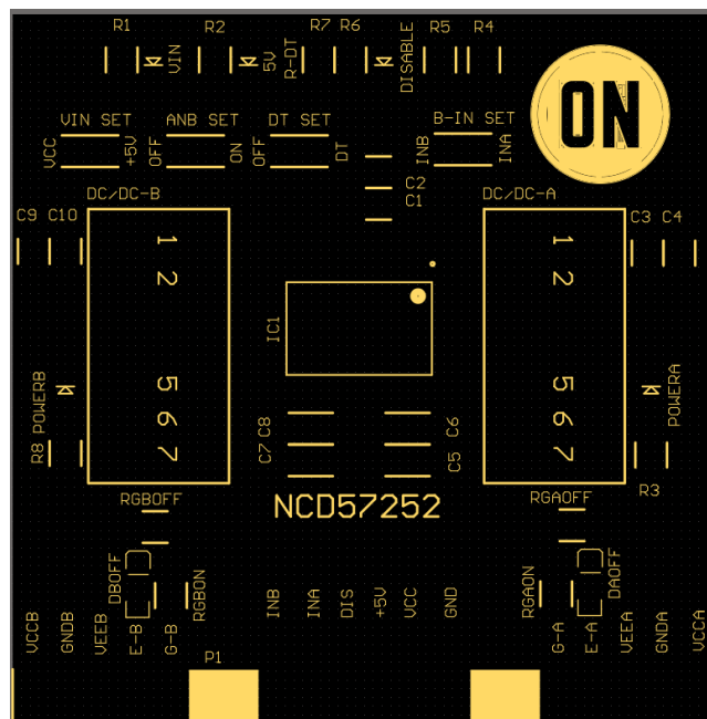
Figure 16. TOP Overlay
