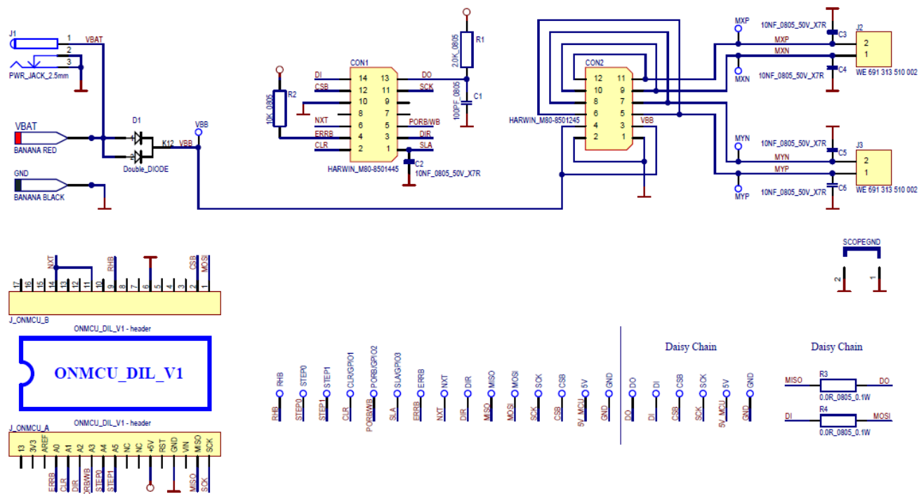
Figure 6. Schematic of SPI Stepper Driver EVK Mother Board
