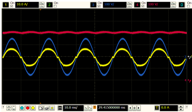
Figure 18. V_{in} = 90\text{ V} , P_{in} = 660\text{ W}
