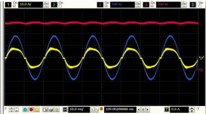
Figure 19. V_{in} = 120\text{ V} , P_{in} = 660\text{ W}
