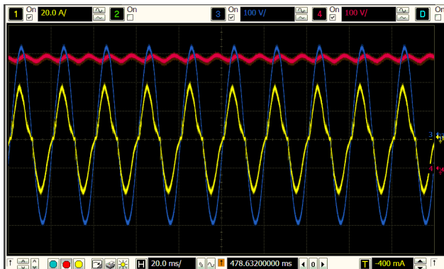
Figure 24. V_{in} = 220\text{ V} , P_{in} = 4.95\text{ kW}
