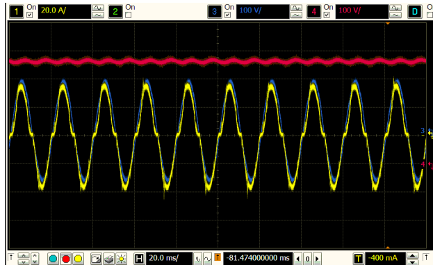
Figure 22. V_{in} = 120\text{ V} , P_{in} = 3.3\text{ kW}
