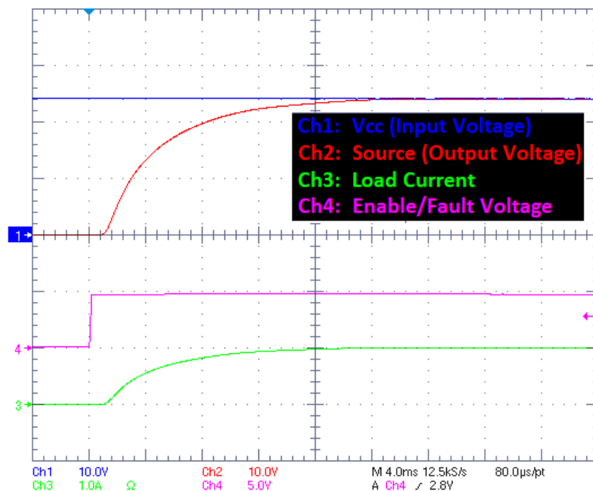
Figure 4. Hot Plug with 180 pF dvdt Capacitor Selected with Jumper Jdvdt into 24 \Omega Load (4 ms/Division Timescale)
