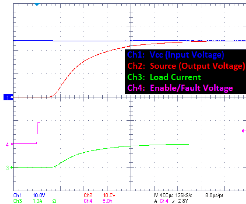
Figure 3. Hot Plug with dvdt Open into 24 \Omega Load (400 \mu s/Division Timescale)
