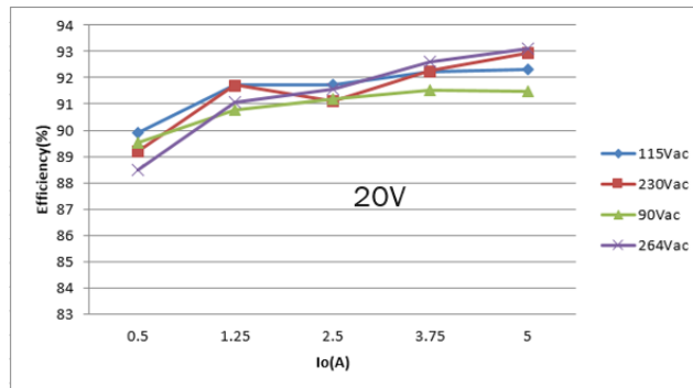
Figure 17. PD_20V Output
