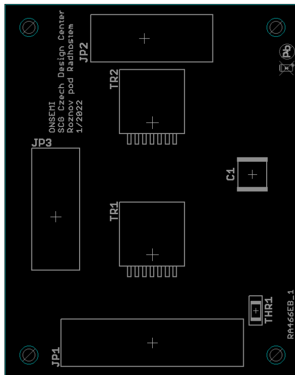
Figure 32. Assembly TOP
