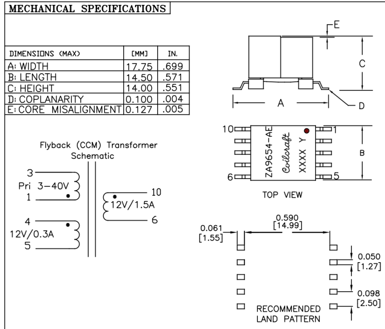
Figure 3. Mechanical Specifications
