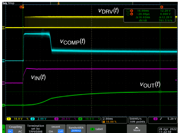
Figure 8. V_{CC} = V_{IN} , V_{IN} = 25\text{ V} , I_{OUT} = 1\text{ A} , t_{\text{startup}} = 16\text{ ms}
