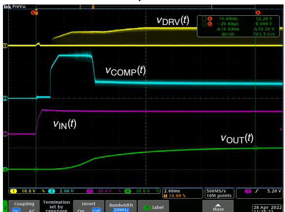
Figure 10. V_{CC} = V_{aux} , V_{IN} = 25\text{ V} , I_{OUT} = 1\text{ A} , t_{\text{startup}} = 16\text{ ms}
