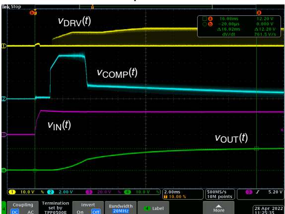
Figure 9. V_{CC} = V_{aux} , V_{IN} = 25\text{ V} , I_{OUT} = 0\text{ A} , t_{\text{startup}} = 16\text{ ms}
