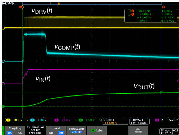
Figure 7. V_{CC} = V_{IN} , V_{IN} = 25\text{ V} , I_{OUT} = 0\text{ A} , t_{\text{startup}} = 16\text{ ms}
