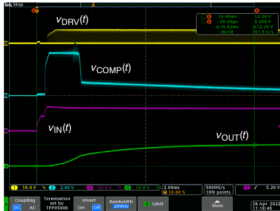
Figure 5. Self-supplied, V_{IN} = 25\text{ V} , I_{OUT} = 0\text{ A} , t_{\text{startup}} = 16\text{ ms}
