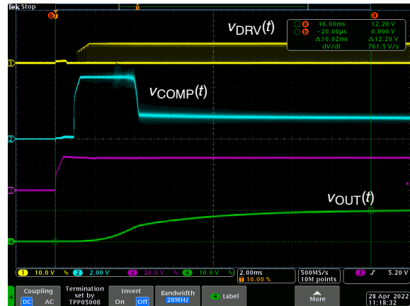
Figure 6. Self-supplied, V_{IN} = 25\text{ V} , I_{OUT} = 1\text{ A} , t_{\text{startup}} = 16\text{ ms}
