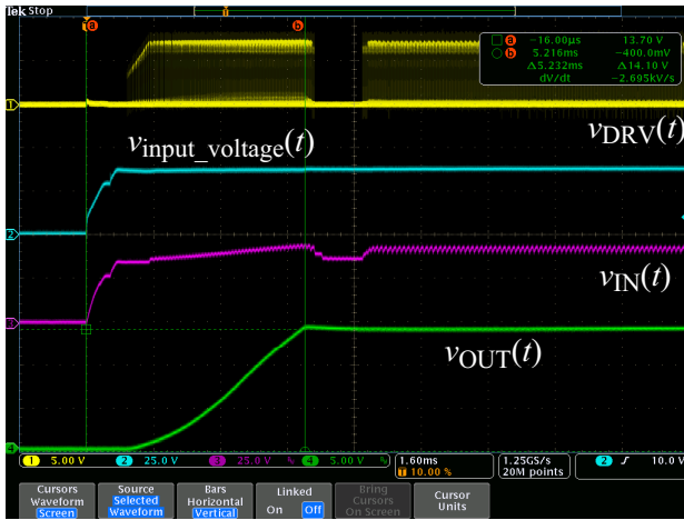
Figure 5. Self-supplied, V_{IN} = 38\text{ V} , I_{OUT} = 0\text{ A} , t_{start} = 5.2\text{ ms}
