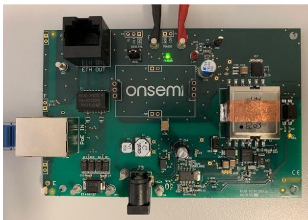
Figure 1. Operational NCP1083REF12VC4GEVB showing Basic Interconnections
