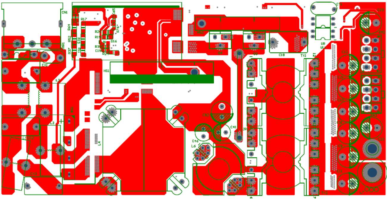
Figure 7. Top View of Mainboard's PCB
