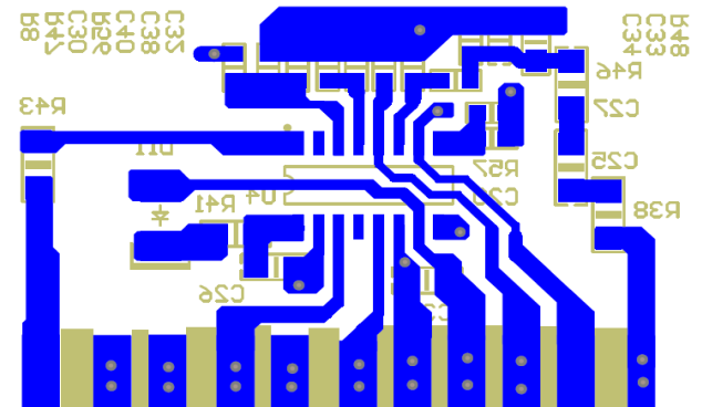
Figure 14. Bottom View of LLC Daughter Card PCB
