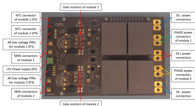
Figure 8. Board Connection
