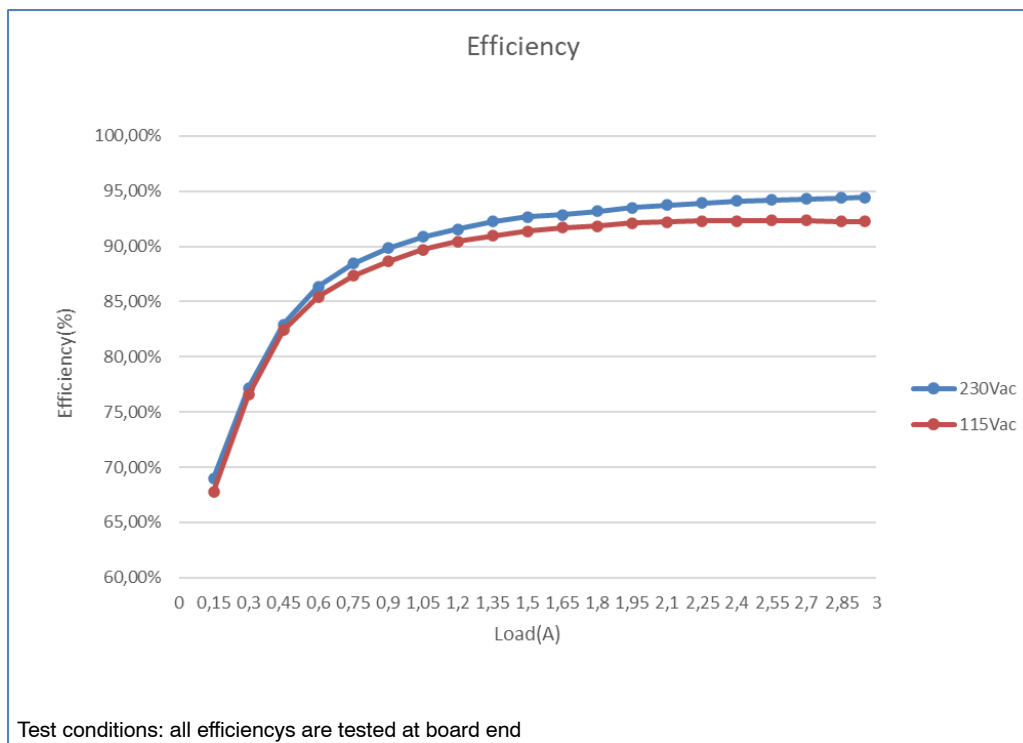
Figure 16. Efficiency Curve
