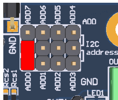
Figure 3. EVB Address Setting (Target Address 0)
