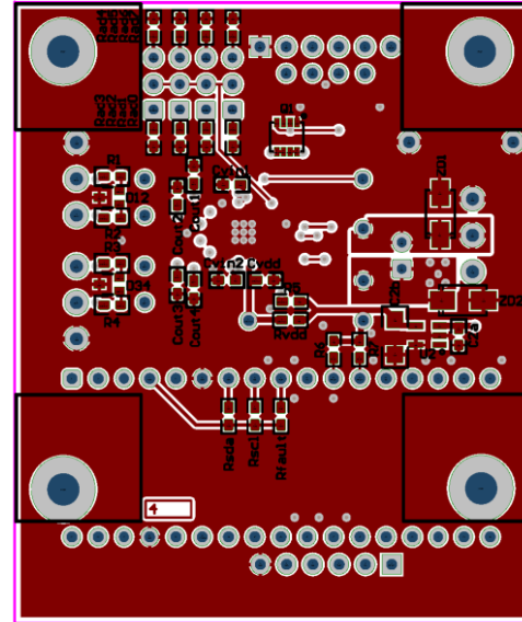
Figure 9. NCV760040 EVB PCB Bottom Composite Drawing (Bottom View)
