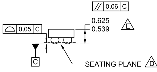
SIDE VIEWS
