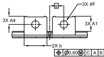
END VIEW
