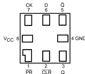
Figure 3. MicorPak™ (Top Through View)
