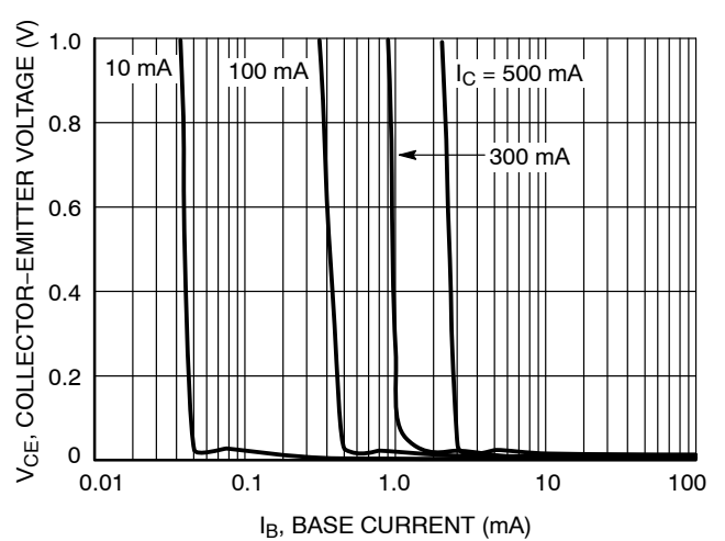
Figure 6. Saturation Region
