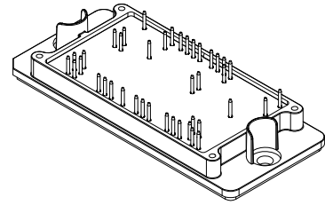
PIM41, 93x47 (SOLDER PIN) CASE 180BC
