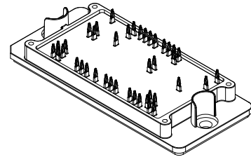
PIM41, 93x47 (PRESS FIT) CASE 180HD
