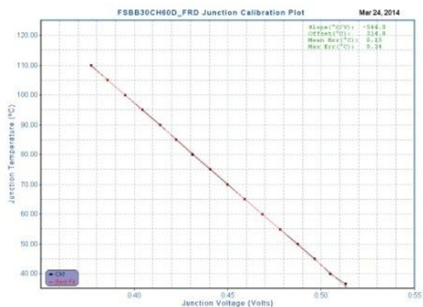
Figure 10. Results of Device Junction Calibration for FRD
