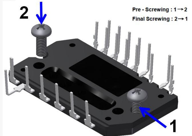
Figure 1. Mounting Screws Fastening Order: Pre-Screwing: 1 → 2; Final Screwing: 2 → 1
