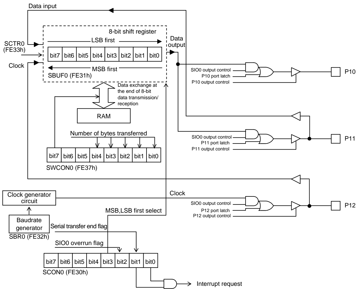
Figure 3.10.2 SIO0 Continuous Data Transmission/Reception Mode Block Diagram (SI0CTR=1)
