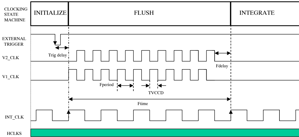
Figure 4. Flush Timing
