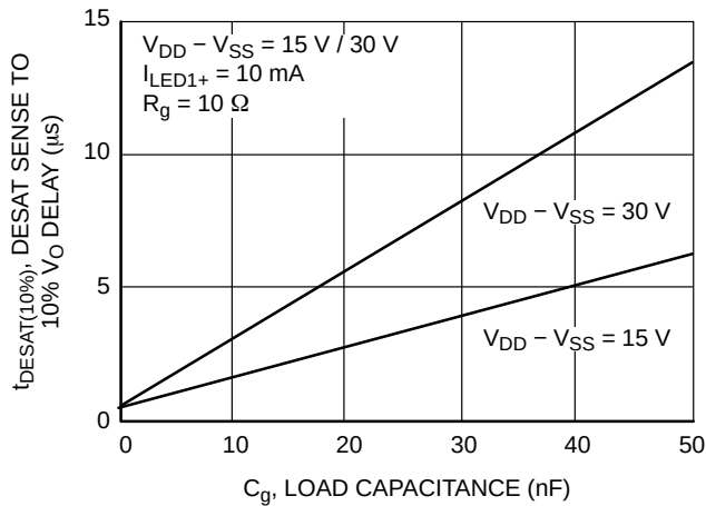
图 25. DESAT Sense to 10% V_O Delay ( t_{\text{DESAT}(10\%)} ) vs. Load Capacitance ( C_g )
