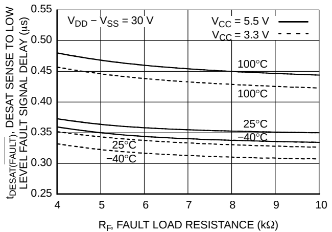
图 26. DESAT Sense to Low Level Fault Signal Delay ( t_{\text{DESAT(FAULT)}} ) vs. Fault Load Resistance ( R_F )
