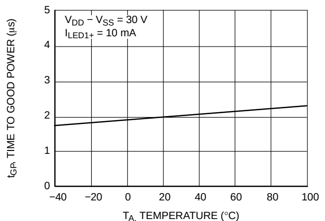
图 28. Time to Good Power ( t_{\text{GP}} ) vs. Temperature
