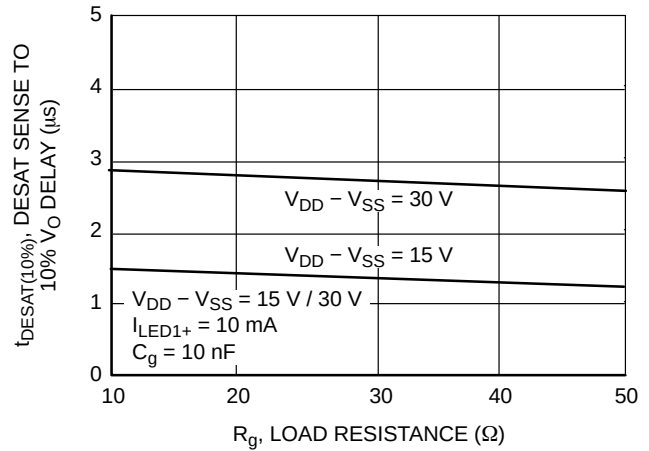
图 24. DESAT Sense to 10% V_O Delay ( t_{\text{DESAT}(10\%)} ) vs. Load Resistance ( R_g )
