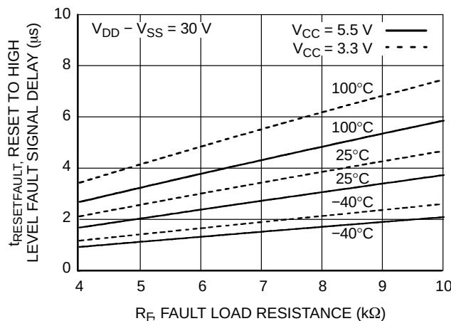
图 27. RESET to High Level Fault Signal Delay ( t_{\text{RESET(FAULT)}} ) vs. Fault Load Resistance ( R_F )
