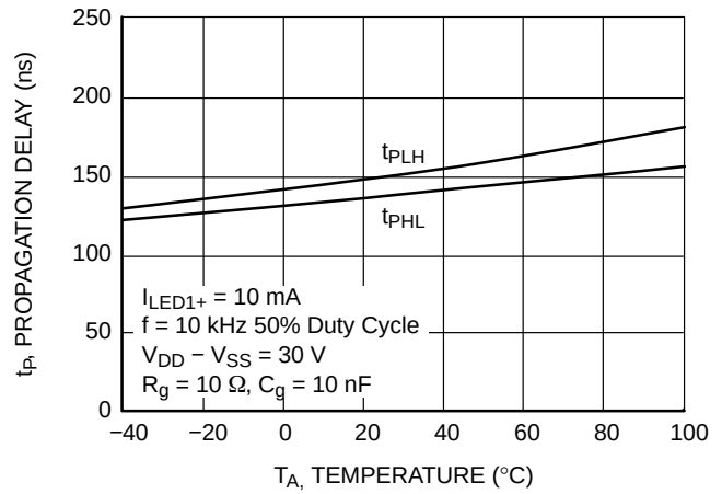
图 18. Propagation Delay ( t_p ) vs. Temperature
