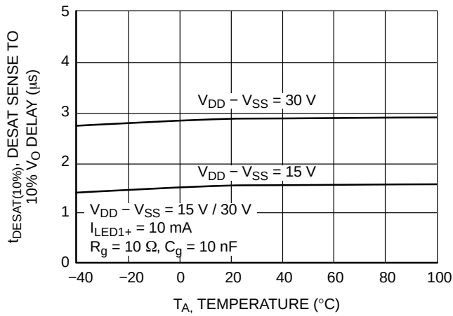
图 23. DESAT Sense to 10% V_O Delay ( t_{\text{DESAT}(10\%)} ) vs. Temperature
