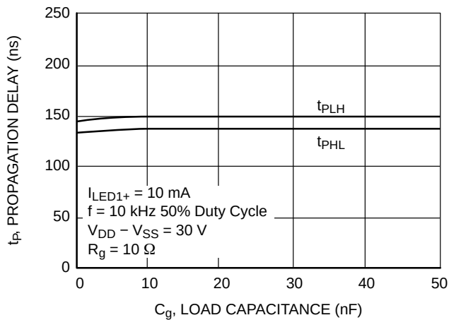
图 21. Propagation Delay ( t_p ) vs. Load Capacitance ( C_g )
