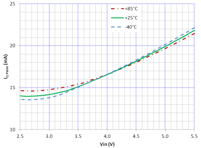
Figure 21. I_{\text{Q PWM}} vs V_{\text{IN}} and Temperature
