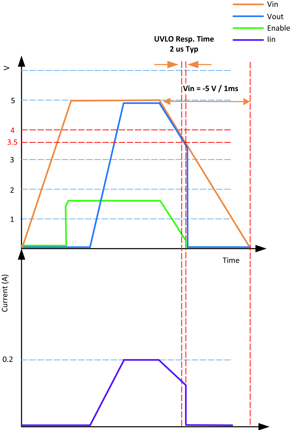
Figure 8. UVLO
