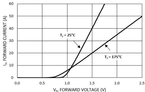
Figure 5. Boost Diode Forward Characteristics
