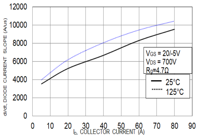
Figure 28. Typical di/dt Current Slope versus I_D
