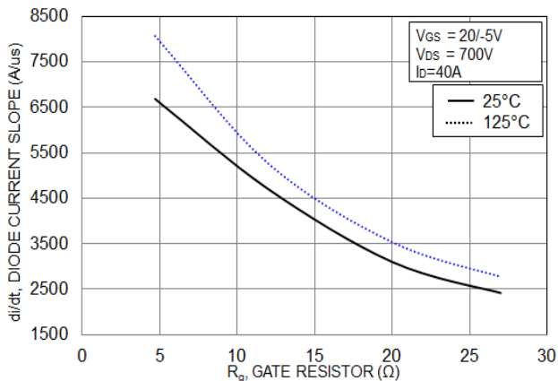
Figure 32. Inverse Diode Typical di/dt vs. R_G
